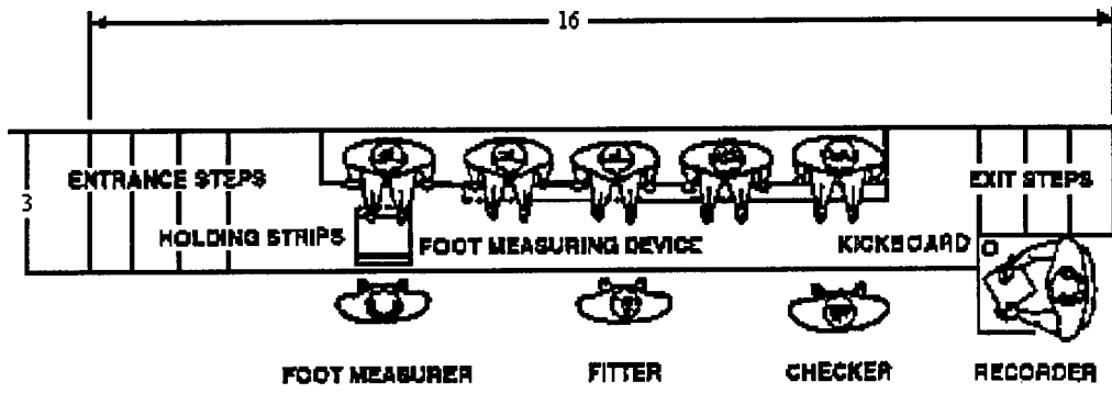
Figure 6-9. Shoe Fitting Platform.
